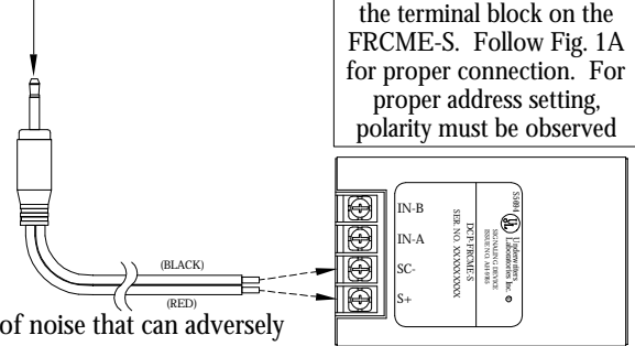
FIGURE 1A. FRCME-S PROGRAMMING CONNECTIONS
